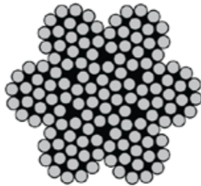
7x19 Galvanised Wire Rope
