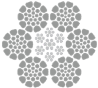
6xK26WS Galvanised Wire Rope
