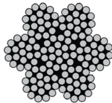
7x19 STAINLESS STEEL WIRE ROPE
