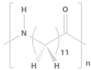
NYLON - 11
